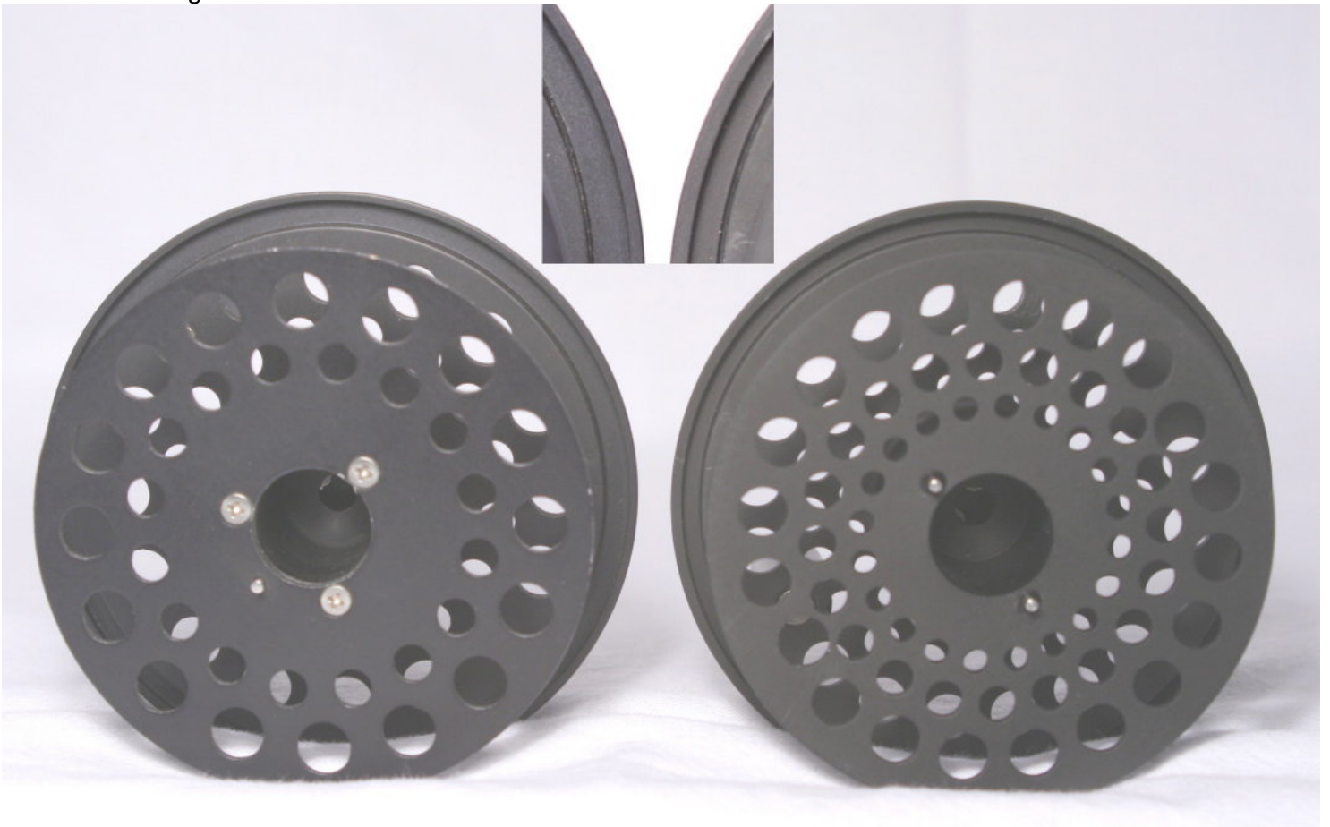
Post 1998 Gunnison Spool – this Spool has two Screws, two Plungers and a Change Ring for Left-Hand wind to Right Hand wind conversion.
